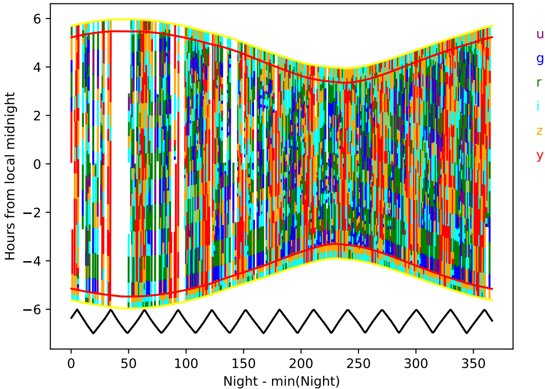
ddf_acor_sf20_lsf30_lsr20_v3.4_10yrs year 6-7: Hourglass
