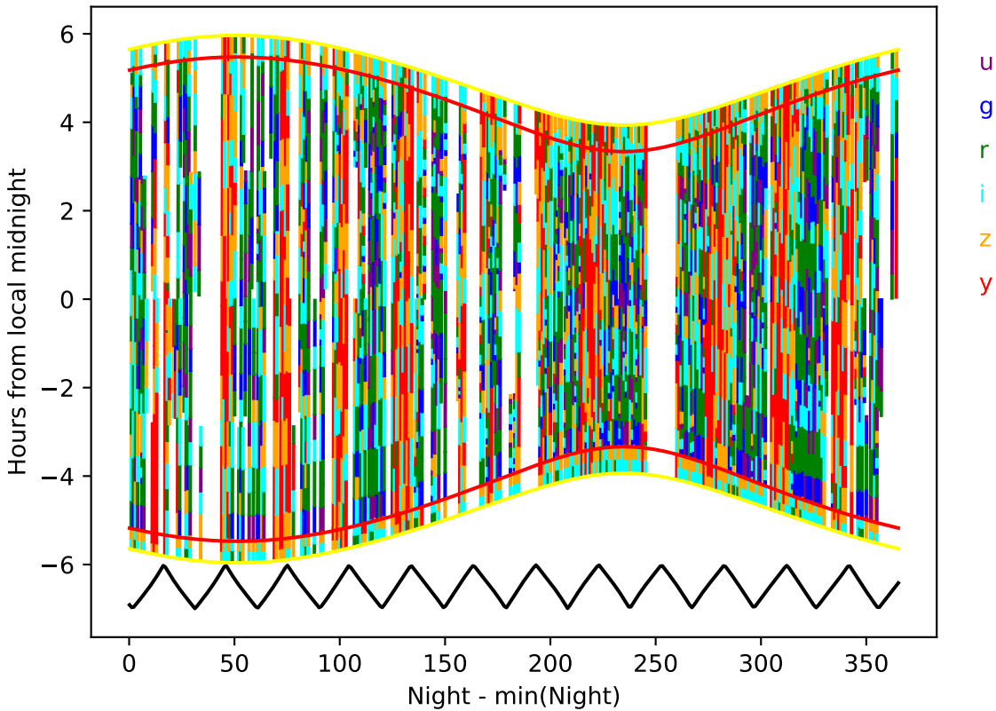
ddf_acor_sf20_lsf30_lsr20_v3.4_10yrs year 5-6: Hourglass
