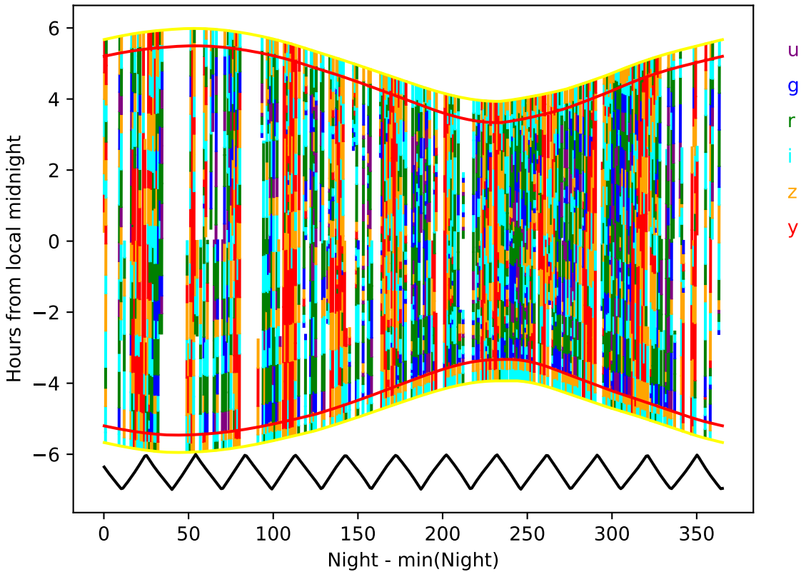
ddf_acor_sf20_lsf30_lsr20_v3.4_10yrs year 4-5: Hourglass
