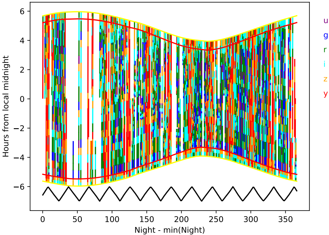
ddf_acor_sf20_lsf30_lsr20_v3.4_10yrs year 3-4: Hourglass
