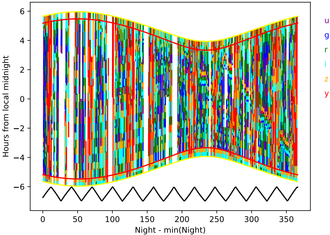
ddf_acor_sf20_ls30_lsr20_v3.4_10yrs year 0-1: Hourglass
