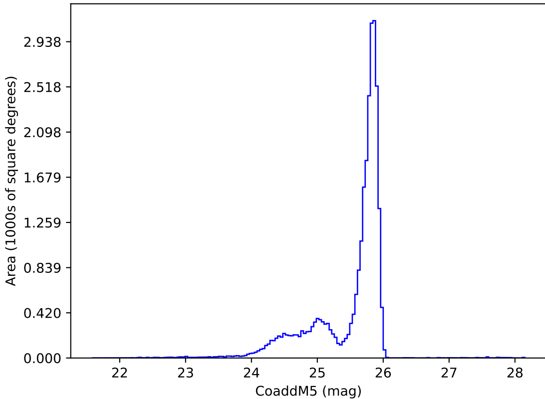
ddf_acor_sf20_lsf30_lsr20_v3.4_10yrs z: CoaddM5
