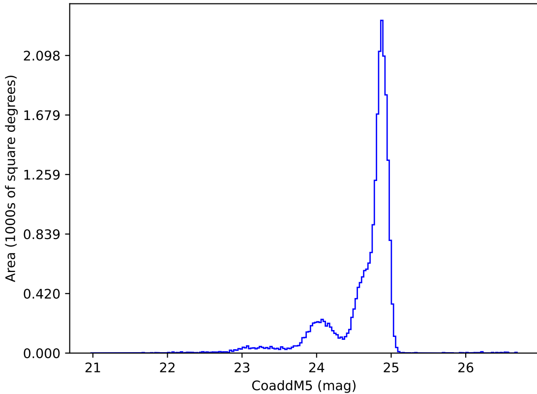
ddf_acor_sf20_lsf30_lsr20_v3.4_10yrs y: CoaddM5
