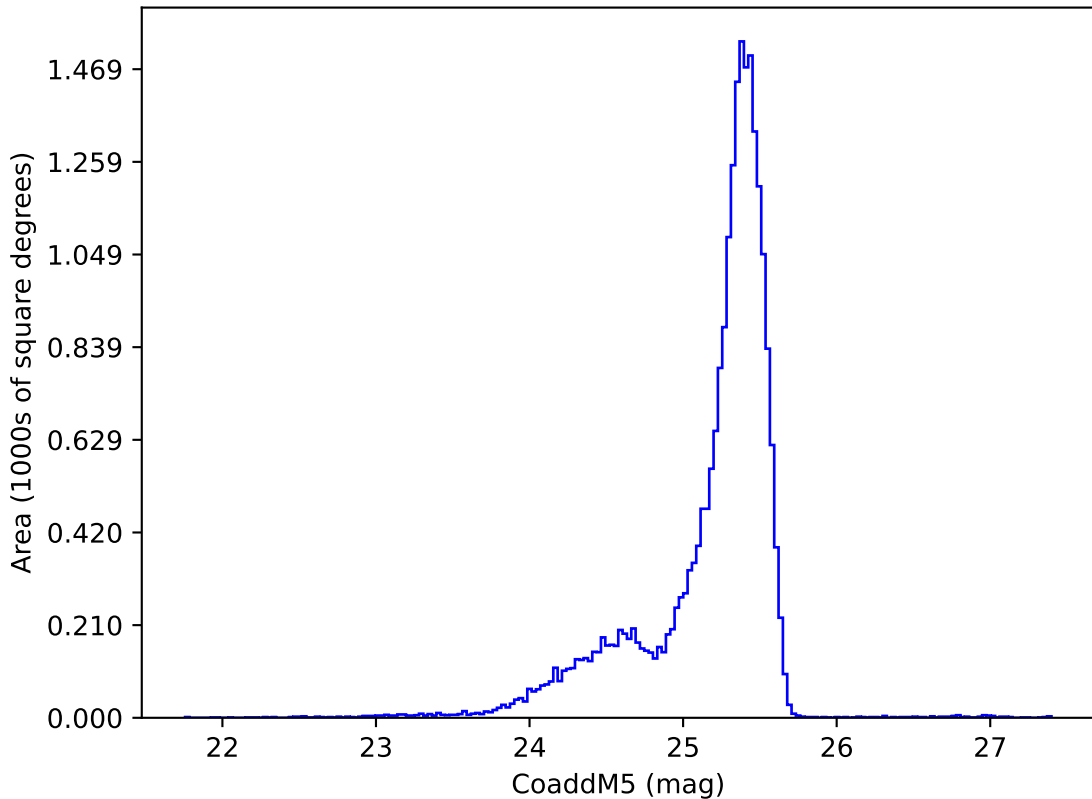
ddf_acor_sf20_lsf30_lsr20_v3.4_10yrs u: CoaddM5
