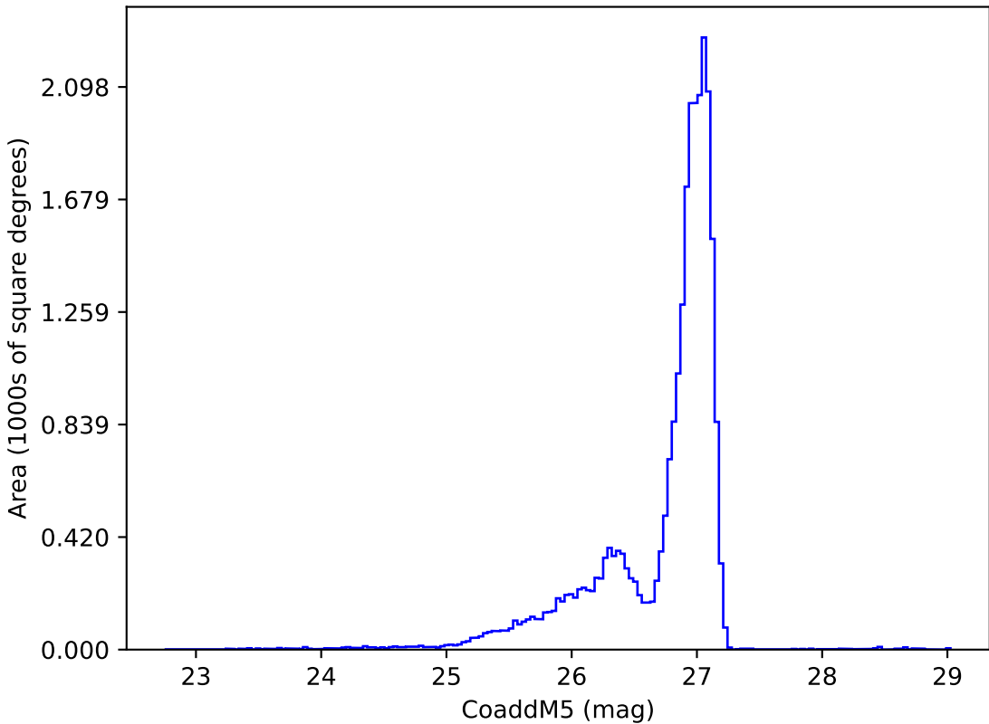
ddf_acor_sf20_lsf30_lsr20_v3.4_10yrs r: CoaddM5
