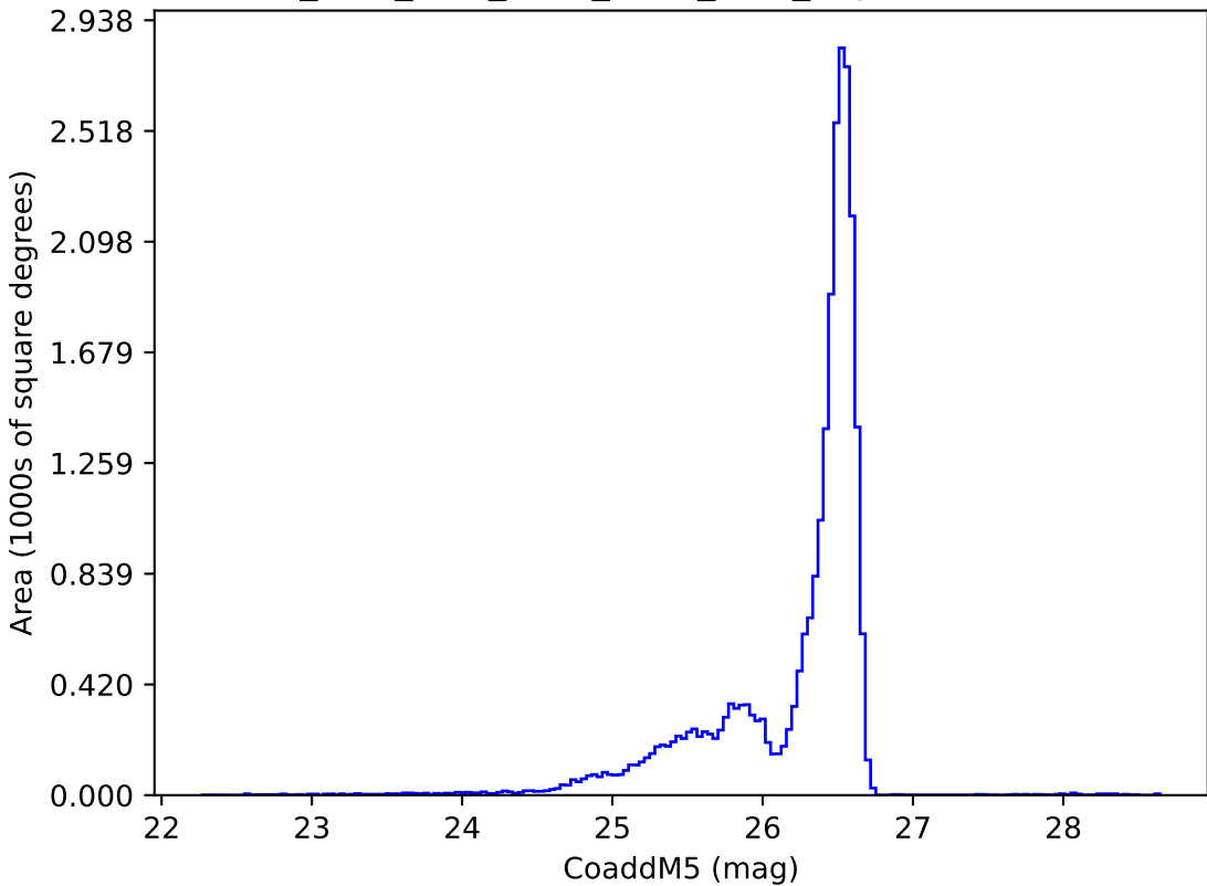
ddf_acor_sf20_lsf30_lsr20_v3.4_10yrs i: CoaddM5
