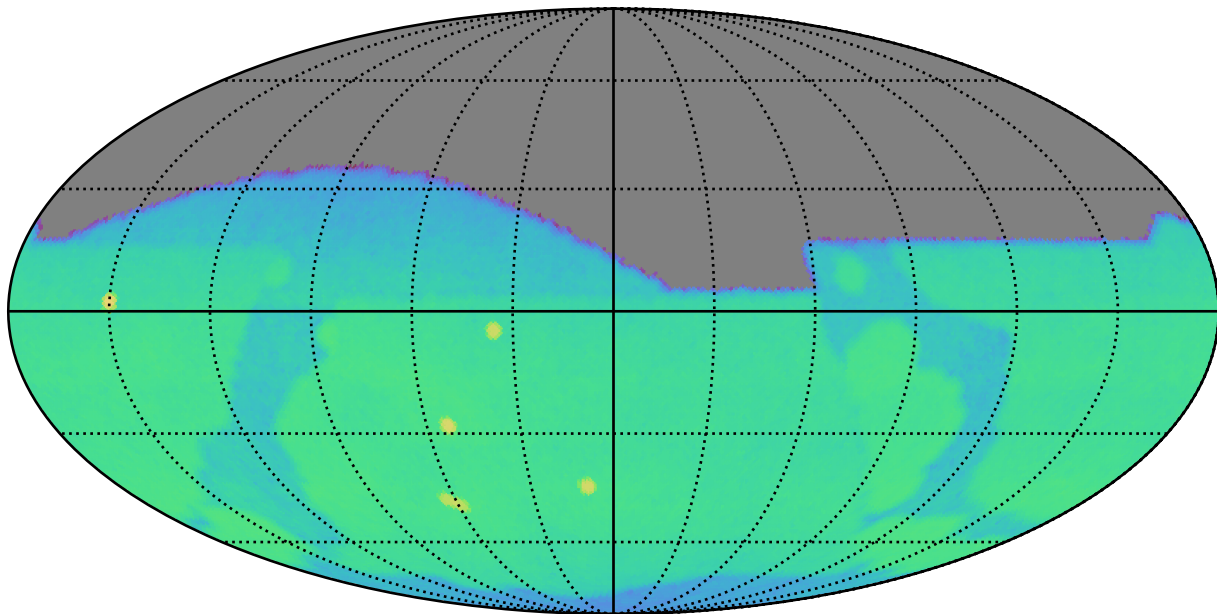
ddf_acor_sf20_lsf30_lsr20_v3.4_10yrs g: CoaddM5
