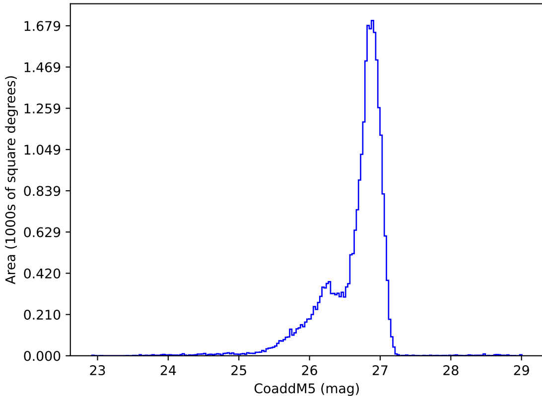
ddf_acor_sf20_lsf30_lsr20_v3.4_10yrs g: CoaddM5
