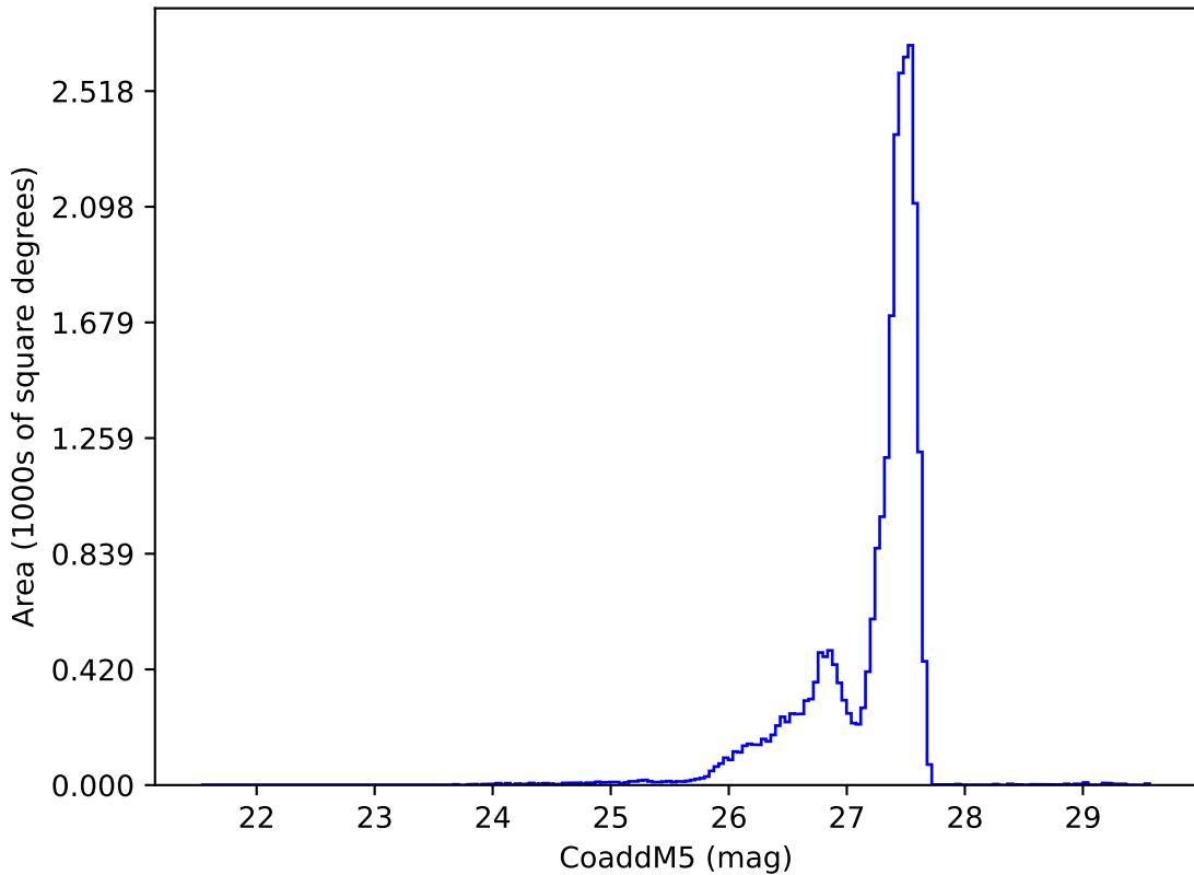
ddf_acor_sf20_lsf30_lsr20_v3.4_10yrs : CoaddM5
