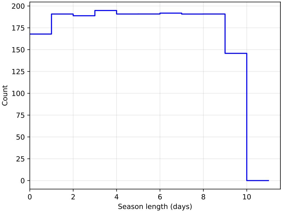
ddf_acor_sf20_lsf30_lsr20_v3.4_10yrs DD:EDFS all bands: SeasonLength
