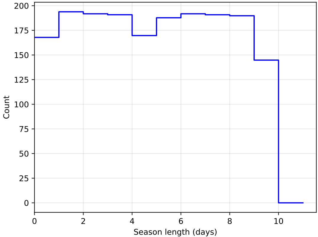
ddf_acor_sf20_lsf30_lsr20_v3.4_10yrs DD:ECDFS all bands: SeasonLength
