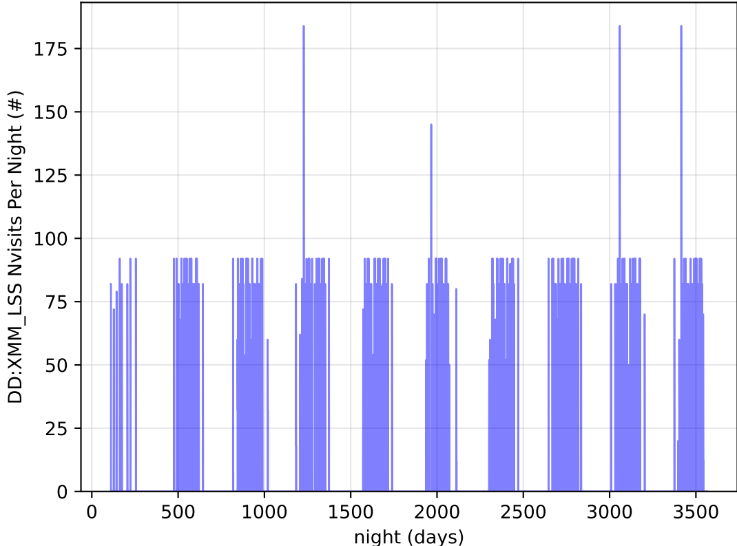
ddf_acor_sf20_lsf30_lsr20_v3.4_10yrs all bands: DD:XMM_LSS Nvisits Per Night
