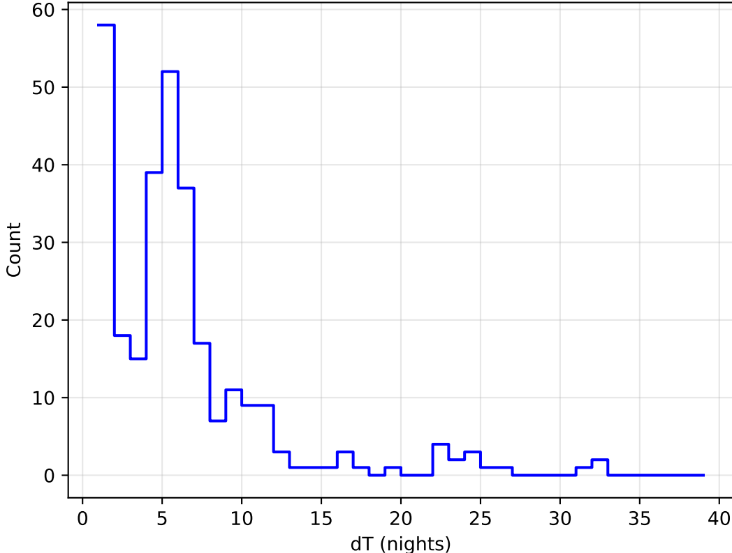
ddf_acor_sf20_Isf30_Isr20_v3.4_10yrs all bands: DD:XMM_LSS Delta Nights Histogram
