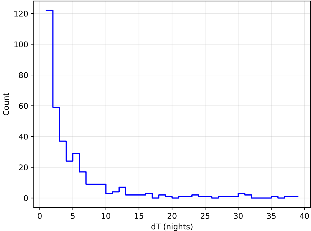
ddf_acor_sf20_lsf30_lsr20_v3.4_10yrs all bands: DD:WFD Delta Nights Histogram
