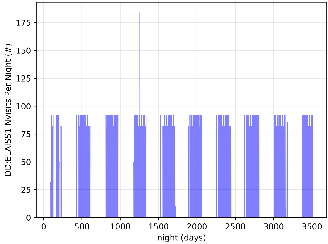
ddf_acor_sf20_lsf30_lsr20_v3.4_10yrs all bands: DD:ELAISS1 Nvisits Per Night
