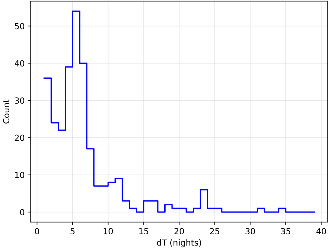
ddf_acor_sf20_lsf30_lsr20_v3.4_10yrs all bands: DD:ELAISS1 Delta Nights Histogram
