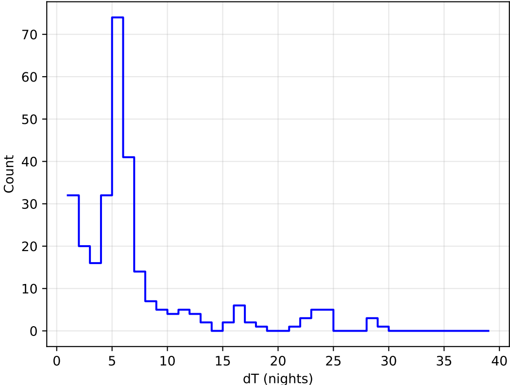
ddf_acor_sf20_lsf30_lsr20_v3.4_10yrs all bands: DD:EDFS Delta Nights Histogram
