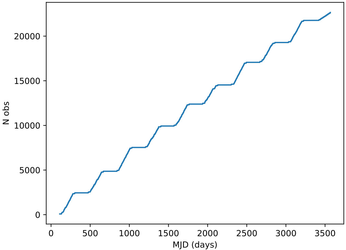
ddf_acor_sf20_lsf30_lsr20_v3.4_10yrs all bands: DD:EDFS Cumulative NVisits
