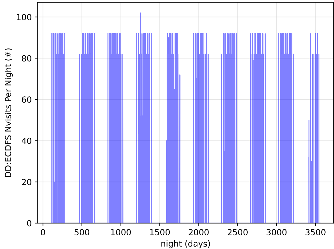
ddf_acor_sf20_lsf30_lsr20_v3.4_10yrs all bands: DD:ECDFS Nvisits Per Night
