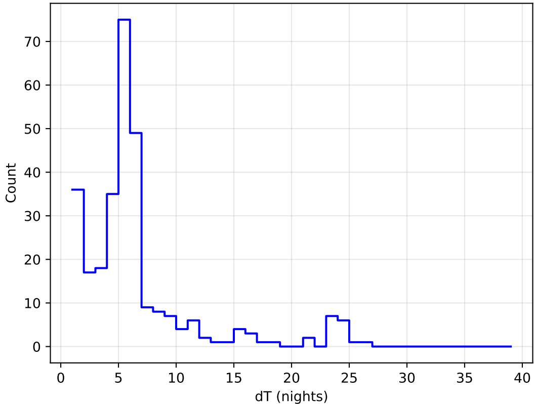
ddf_acor_sf20_lsf30_lsr20_v3.4_10yrs all bands: DD:ECDFS Delta Nights Histogram
