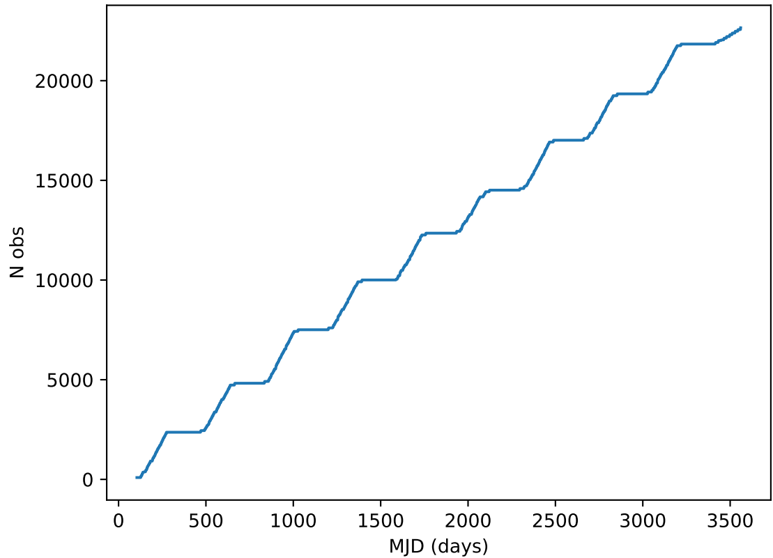
ddf_acor_sf20_lsf30_lsr20_v3.4_10yrs all bands: DD:ECDFS Cumulative NVisits
