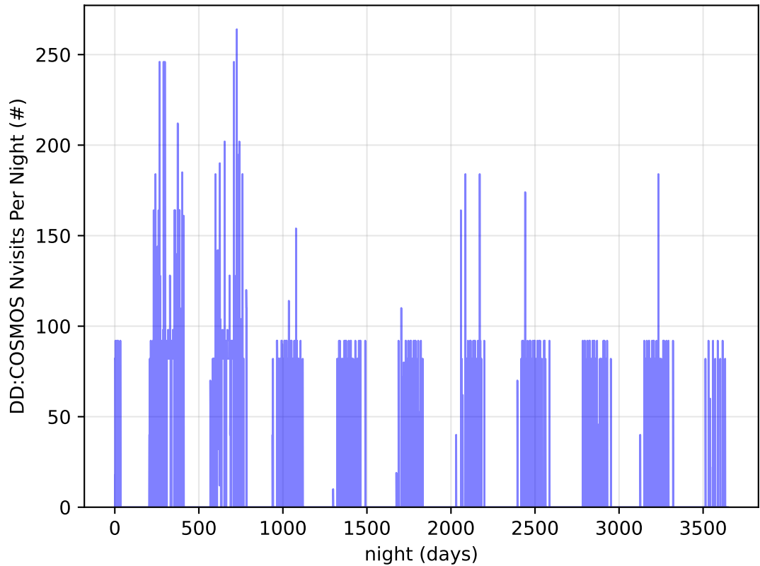
ddf_acor_sf20_lsf30_lsr20_v3.4_10yrs all bands: DD: COSMOS Nvisits Per Night
