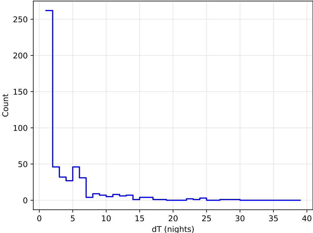
ddf_acor_sf20_Isf30_Isr20_v3.4_10yrs all bands: DD: COSMOS Delta Nights Histogram
