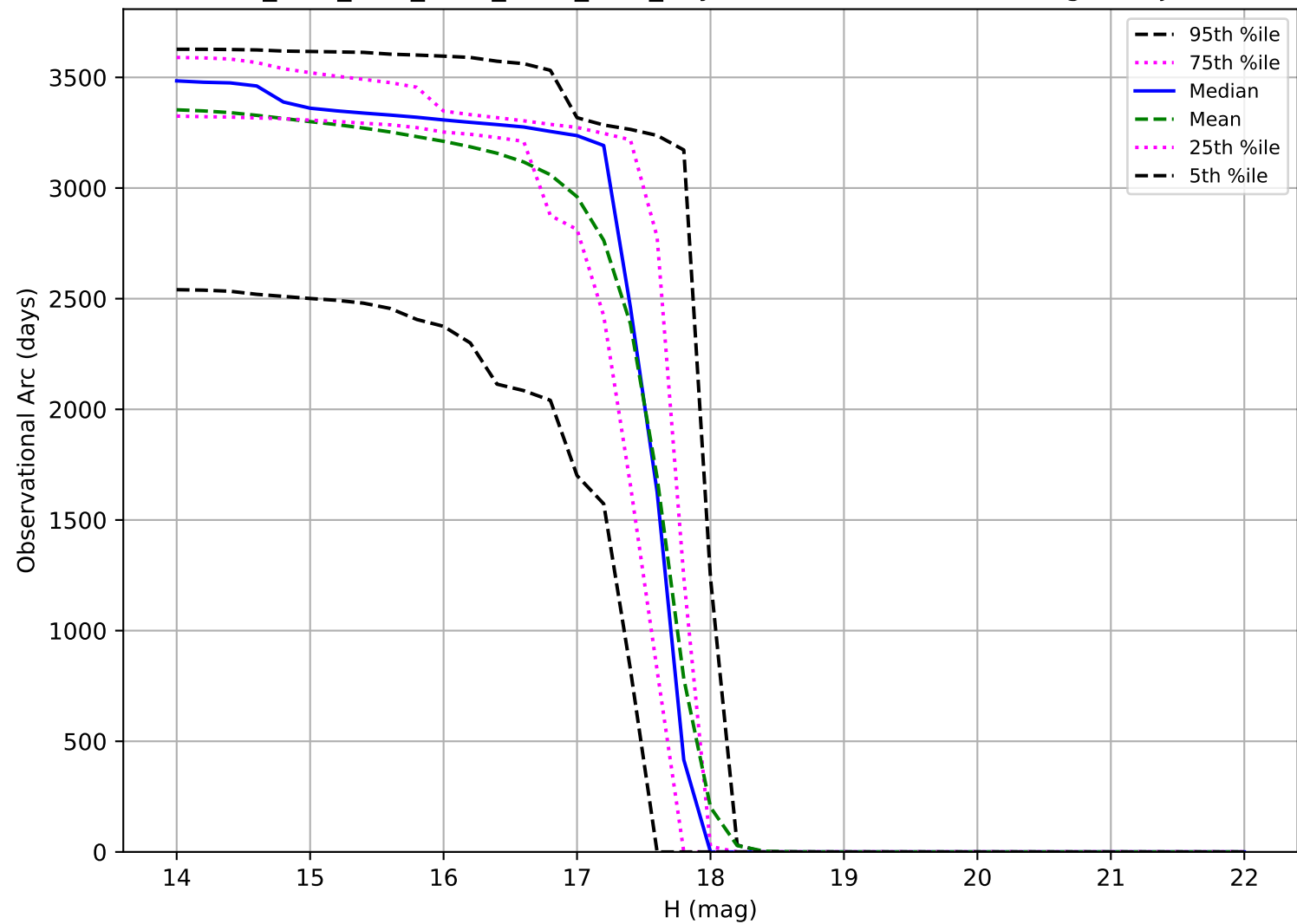
ddf_acor_sf20_lsf30_lsr10_v3.4_10yrs: Observational Arc Length Trojan
