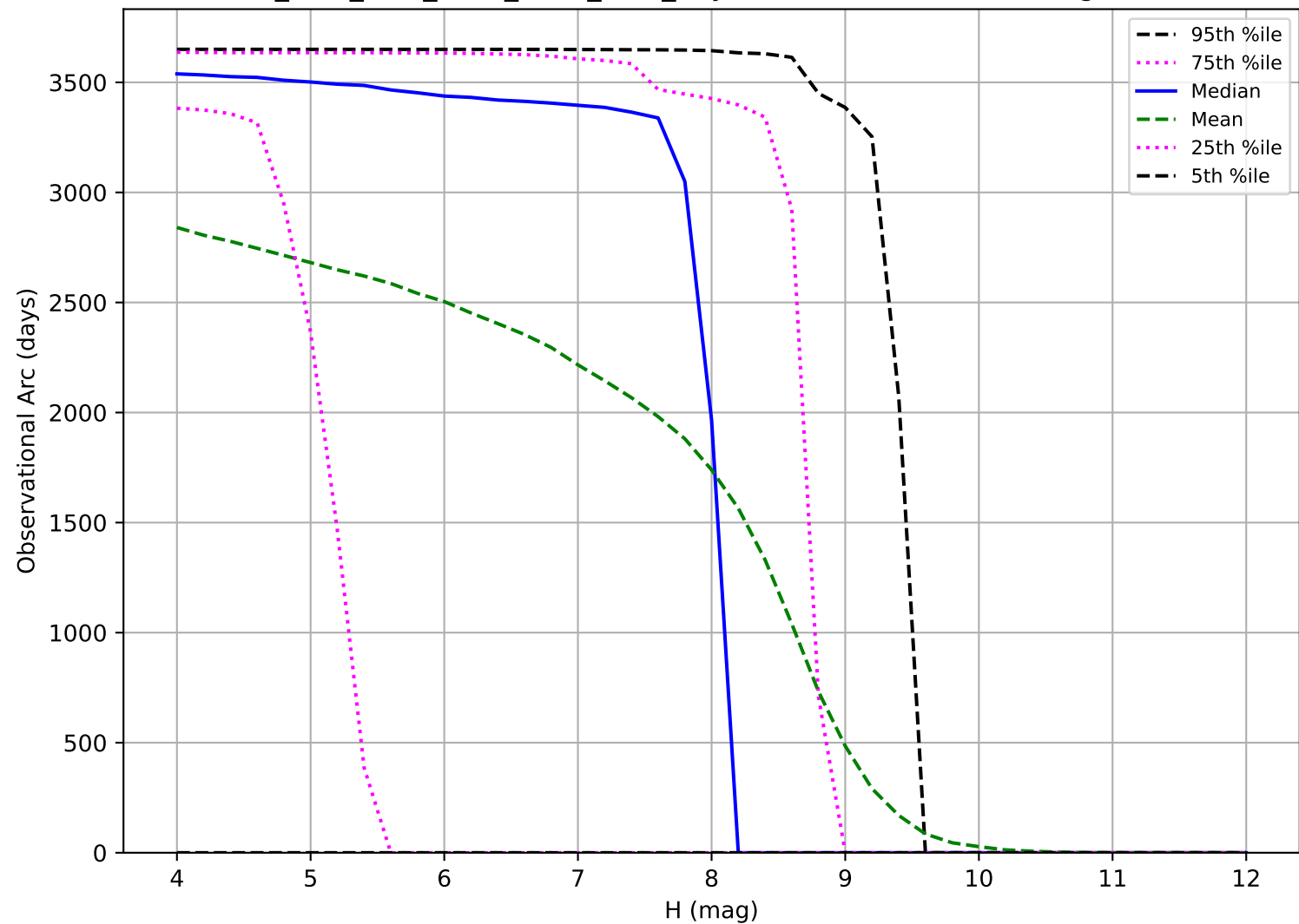
ddf_acor_sf20_lsf30_lsr10_v3.4_10yrs: Observational Arc Length TNO
