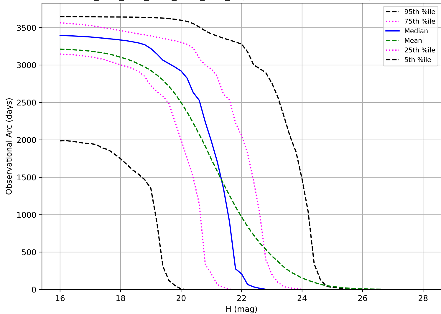
ddf_acor_sf20_lsf30_lsr10_v3.4_10yrs: Observational Arc Length PHA
