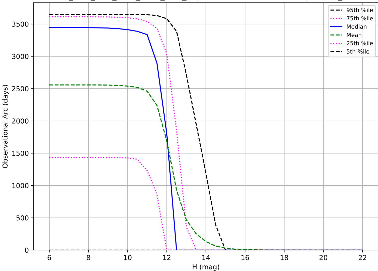
ddf_acor_sf20_lsf30_lsr10_v3.4_10yrs: Observational Arc Length OCC_r20
