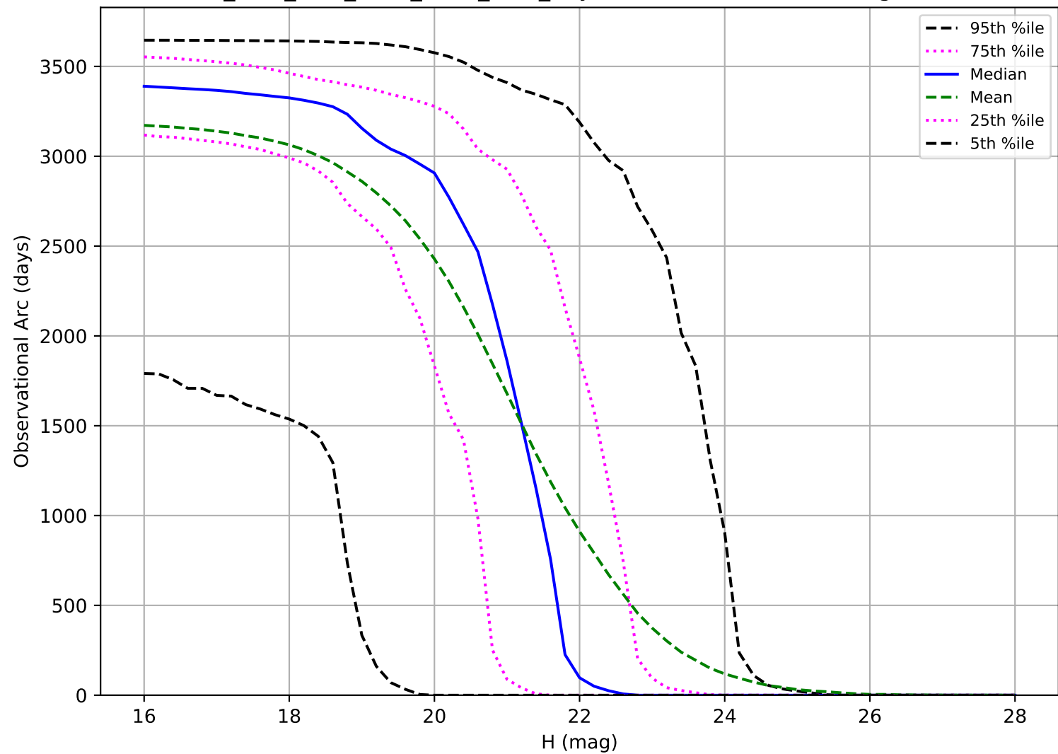
ddf_acor_sf20_lsf30_lsr10_v3.4_10yrs: Observational Arc Length NEO
