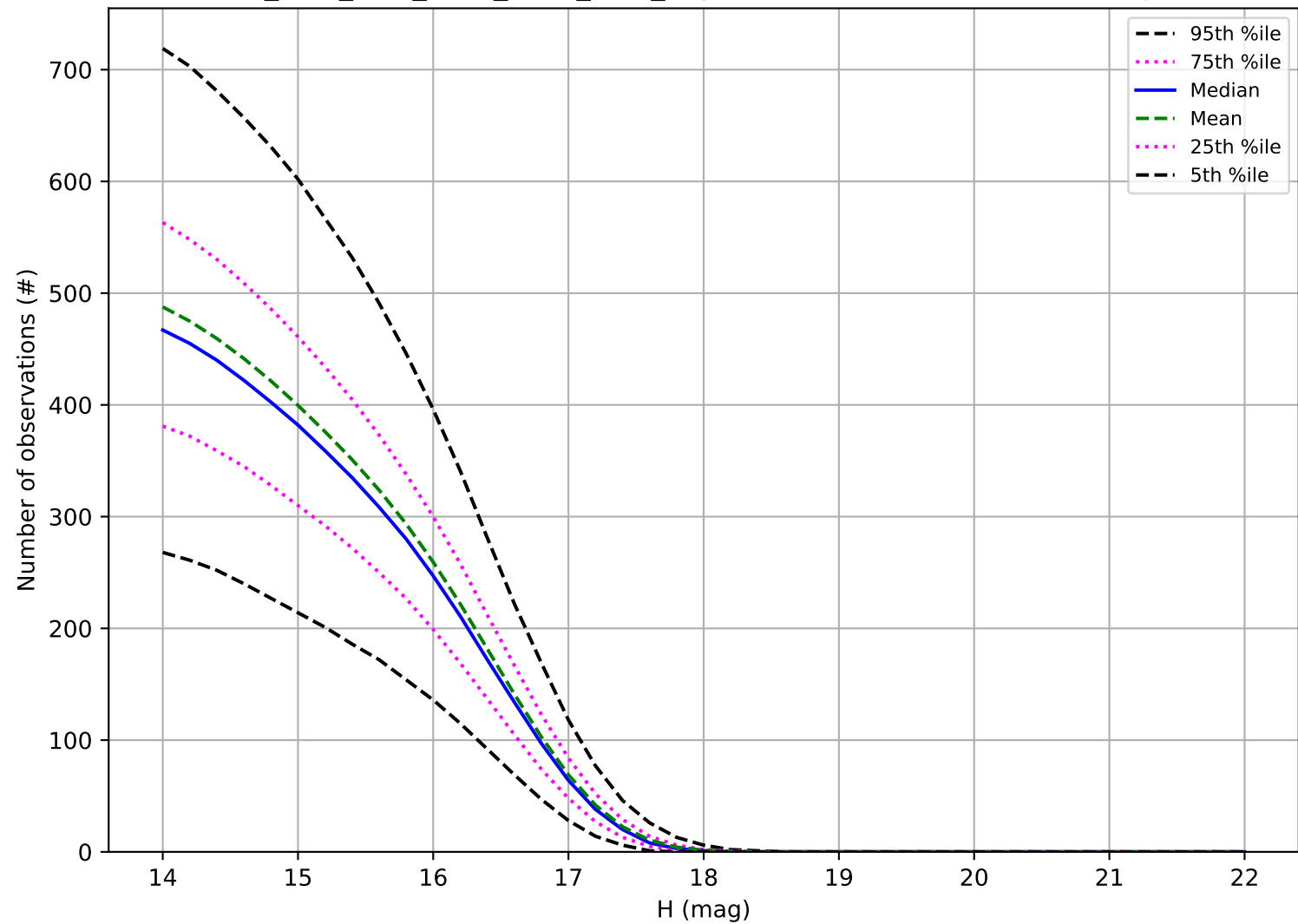
ddf_acor_sf20_lsf30_lsr10_v3.4_10yrs: Number of observations Trojan
