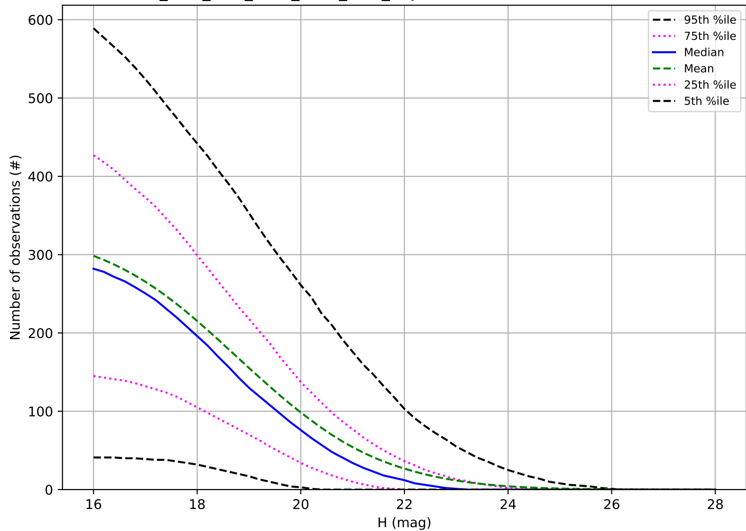
ddf_acor_sf20_lsf30_lsr10_v3.4_10yrs: Number of observations PHA
