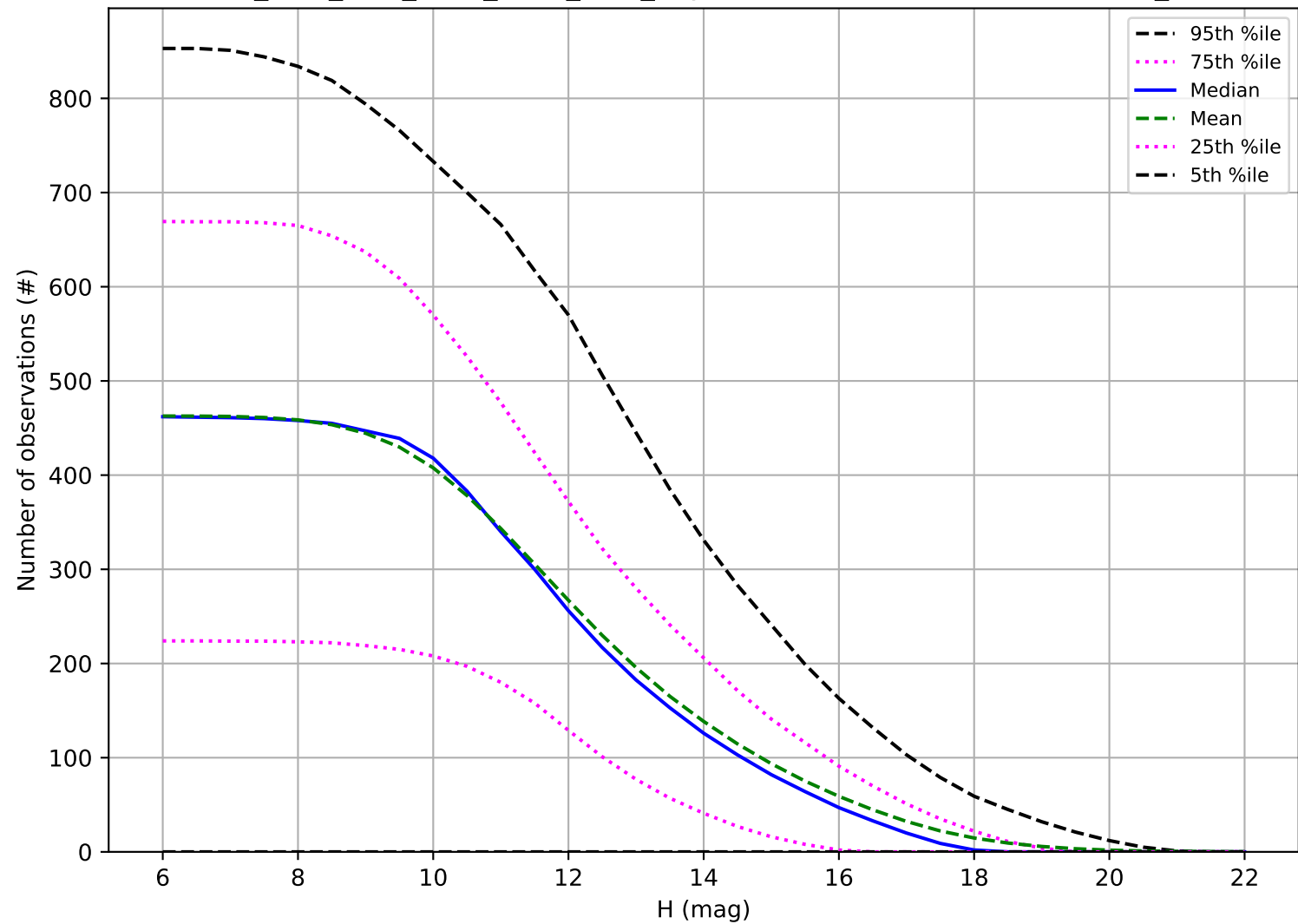
ddf_acor_sf20_lsf30_lsr10_v3.4_10yrs: Number of observations OCC_r5
