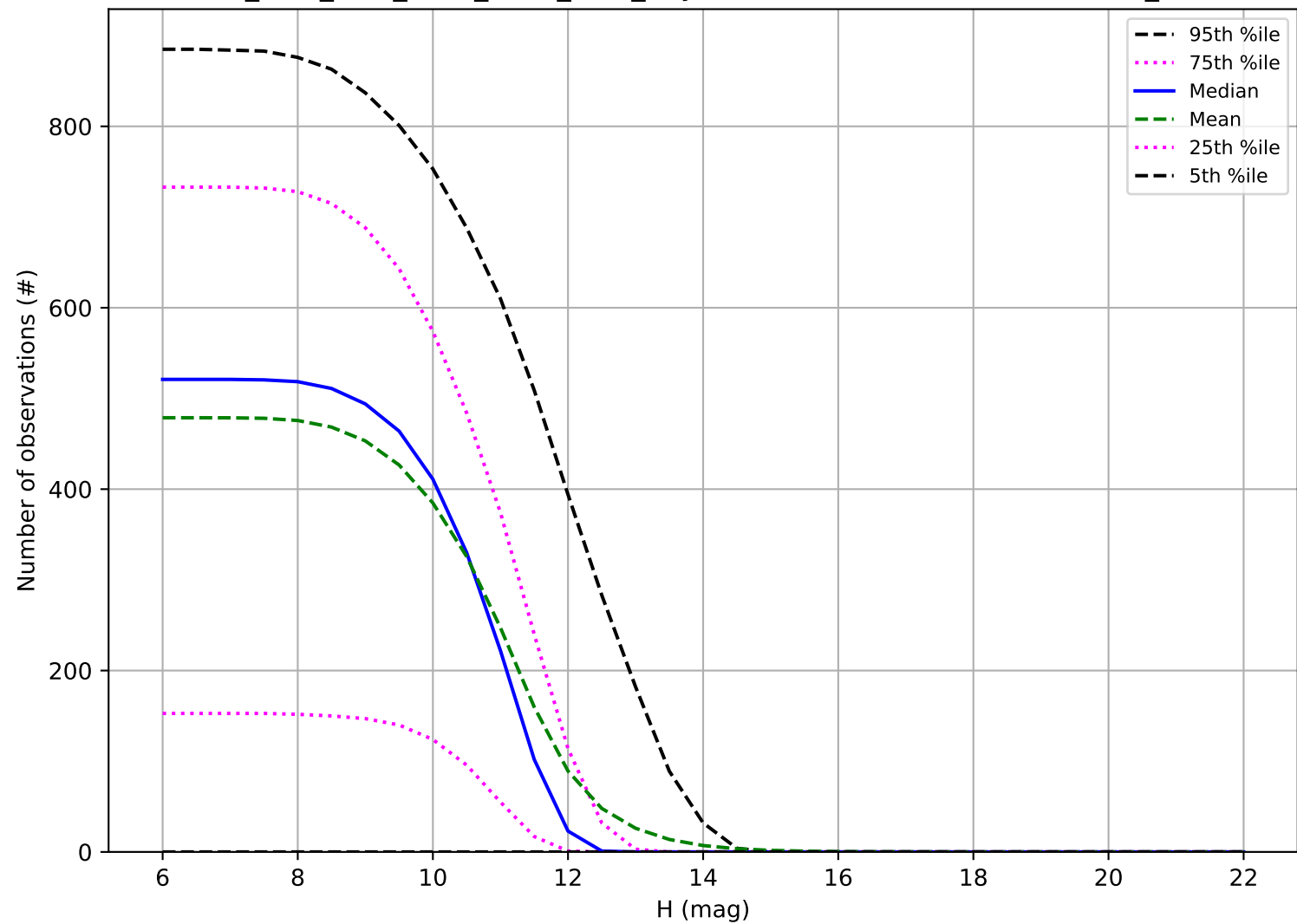
ddf_acor_sf20_lsf30_lsr10_v3.4_10yrs: Number of observations OCC_r20
