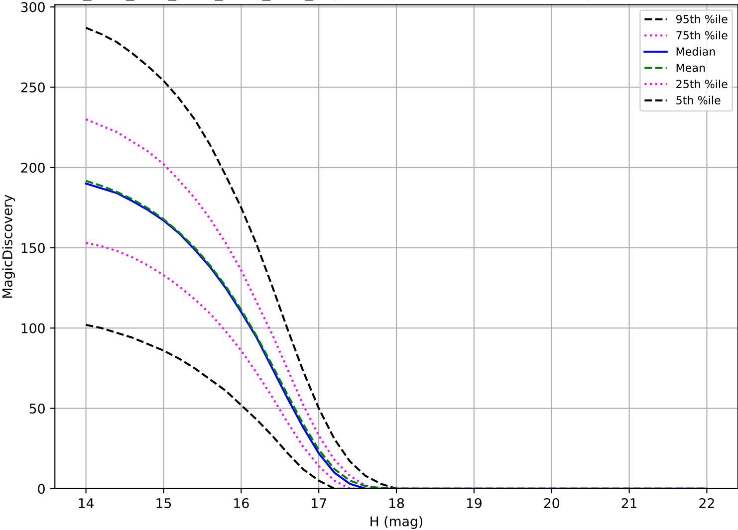
ddf_acor_sf20_lsf30_lsr10_v3.4_10yrs: Trojan 6 detections in 60 nights detection loss
