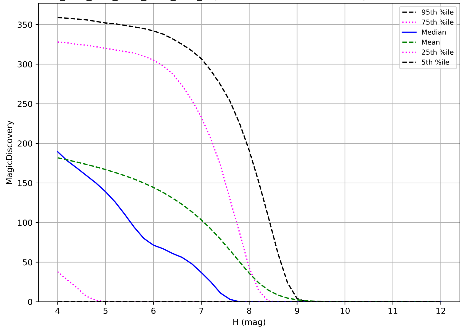
ddf_acor_sf20_lsf30_lsr10_v3.4_10yrs: TNO 6 detections in 60 nights detection loss
