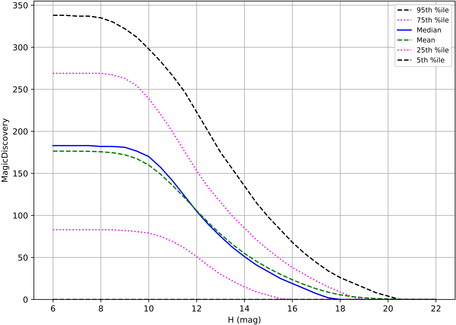
ddf_acor_sf20_lsf30_lsr10_v3.4_10yrs: OCC_r5 6 detections in 60 nights detection loss
