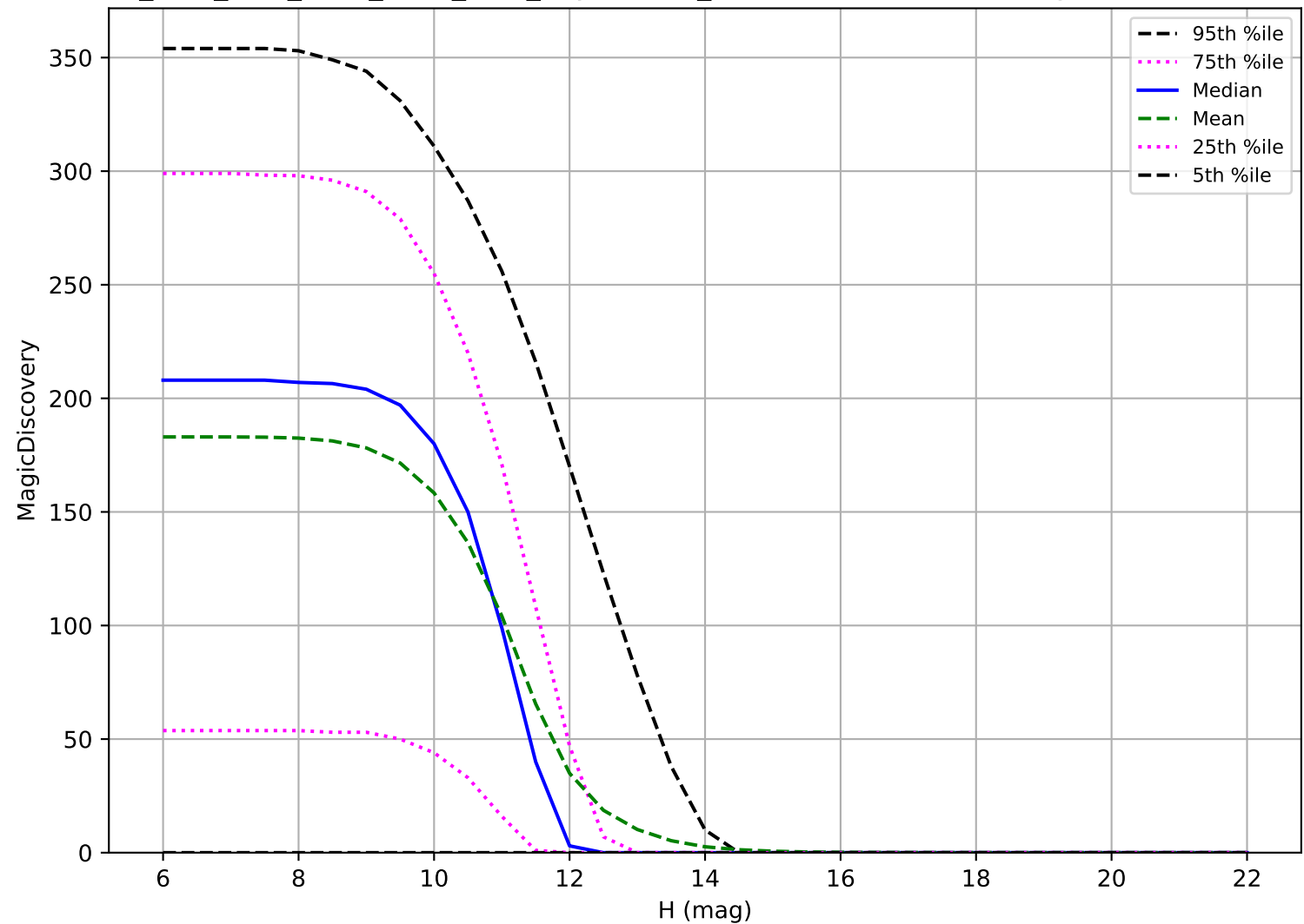
ddf_acor_sf20_lsf30_lsr10_v3.4_10yrs: OCC_r20 6 detections in 60 nights detection loss
