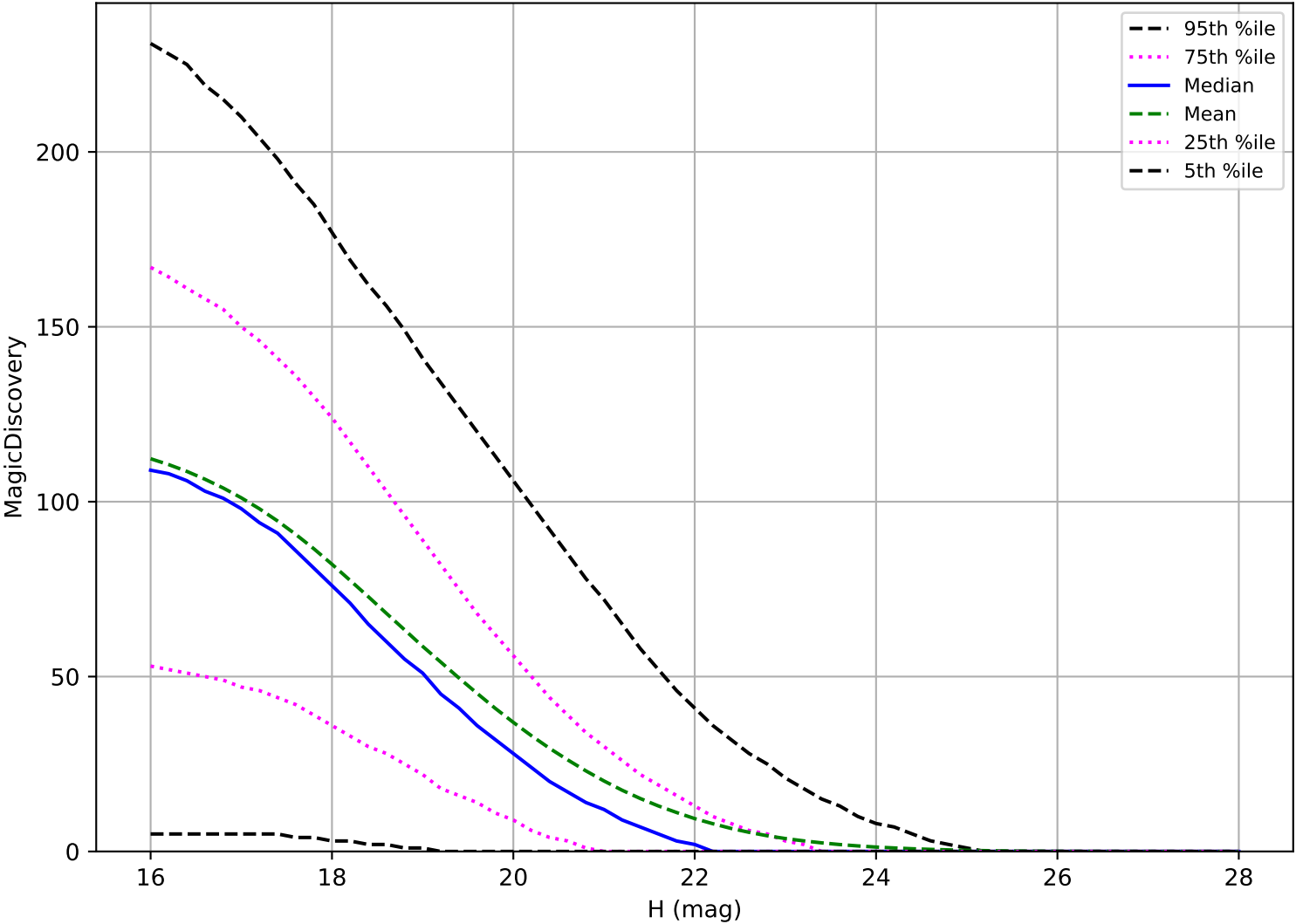
ddf_acor_sf20_lsf30_lsr10_v3.4_10yrs: NEO 6 detections in 60 nights detection loss
