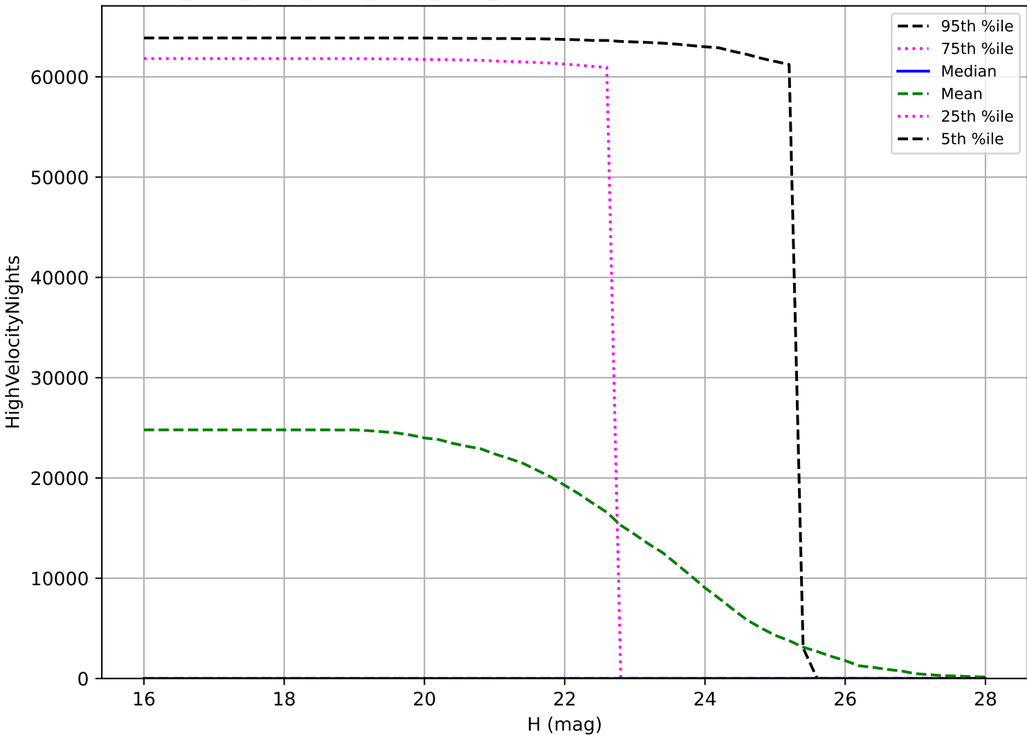
ddf_acor_sf20_lsf30_lsr10_v3.4_10yrs: PHA High velocity pair detection loss
