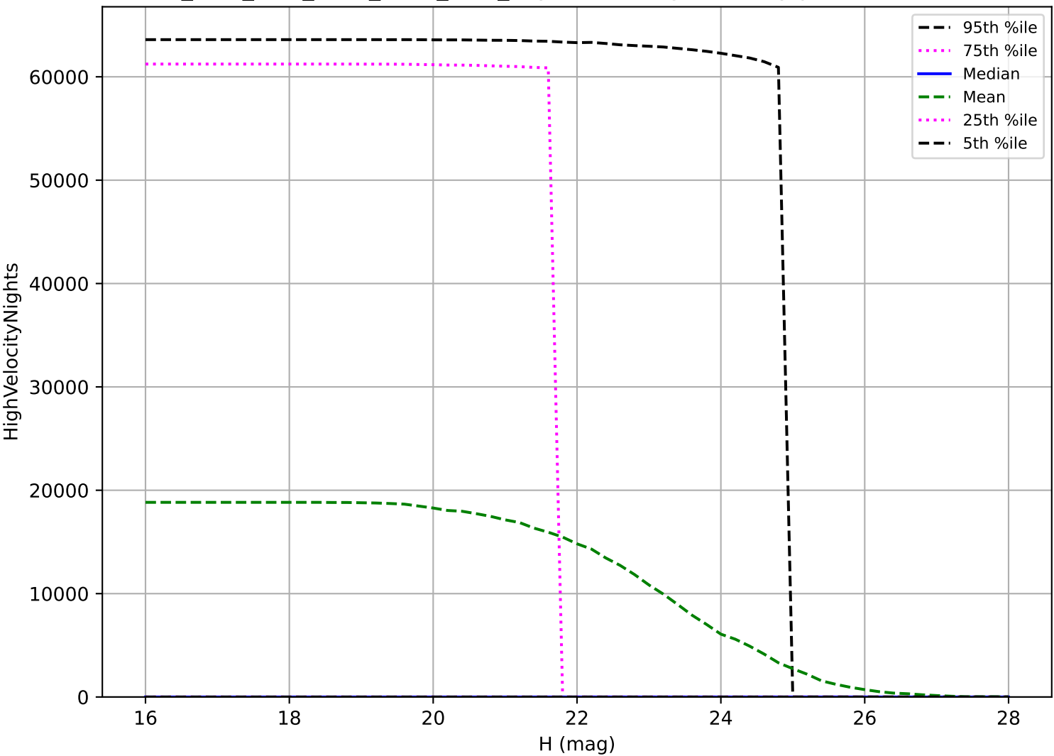
ddf_acor_sf20_lsf30_lsr10_v3.4_10yrs: NEO High velocity pair detection loss
