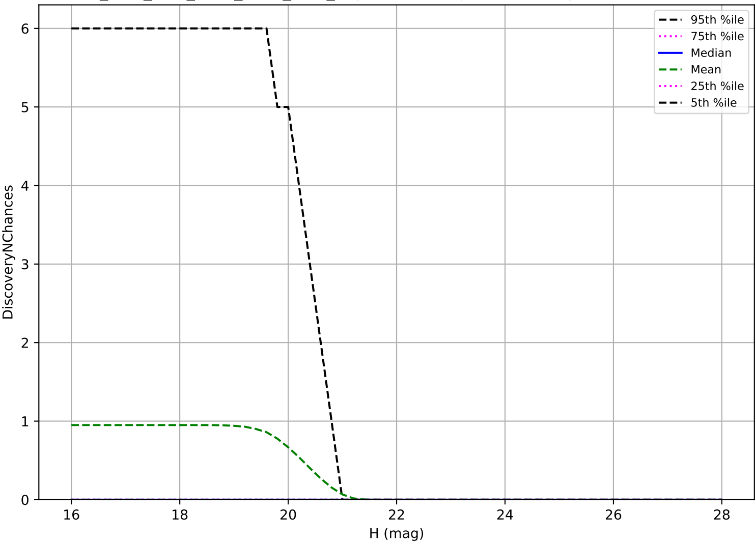
ddf_acor_sf20_lsf30_lsr10_v3.4_10yrs: Vatira 3 pairs in 15 nights detection loss
