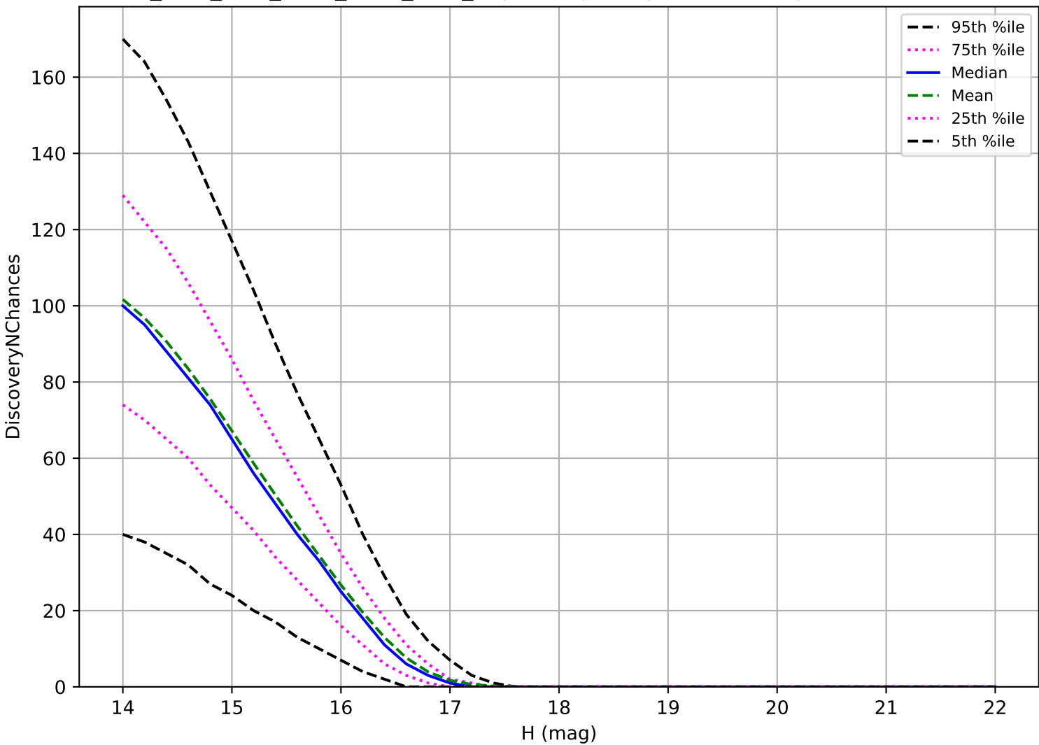
ddf_acor_sf20_lsf30_lsr10_v3.4_10yrs: Trojan 3 pairs in 15 nights detection loss
