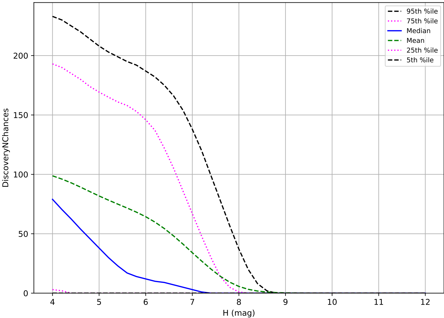
ddf_acor_sf20_lsf30_lsr10_v3.4_10yrs: TNO 3 pairs in 15 nights detection loss
