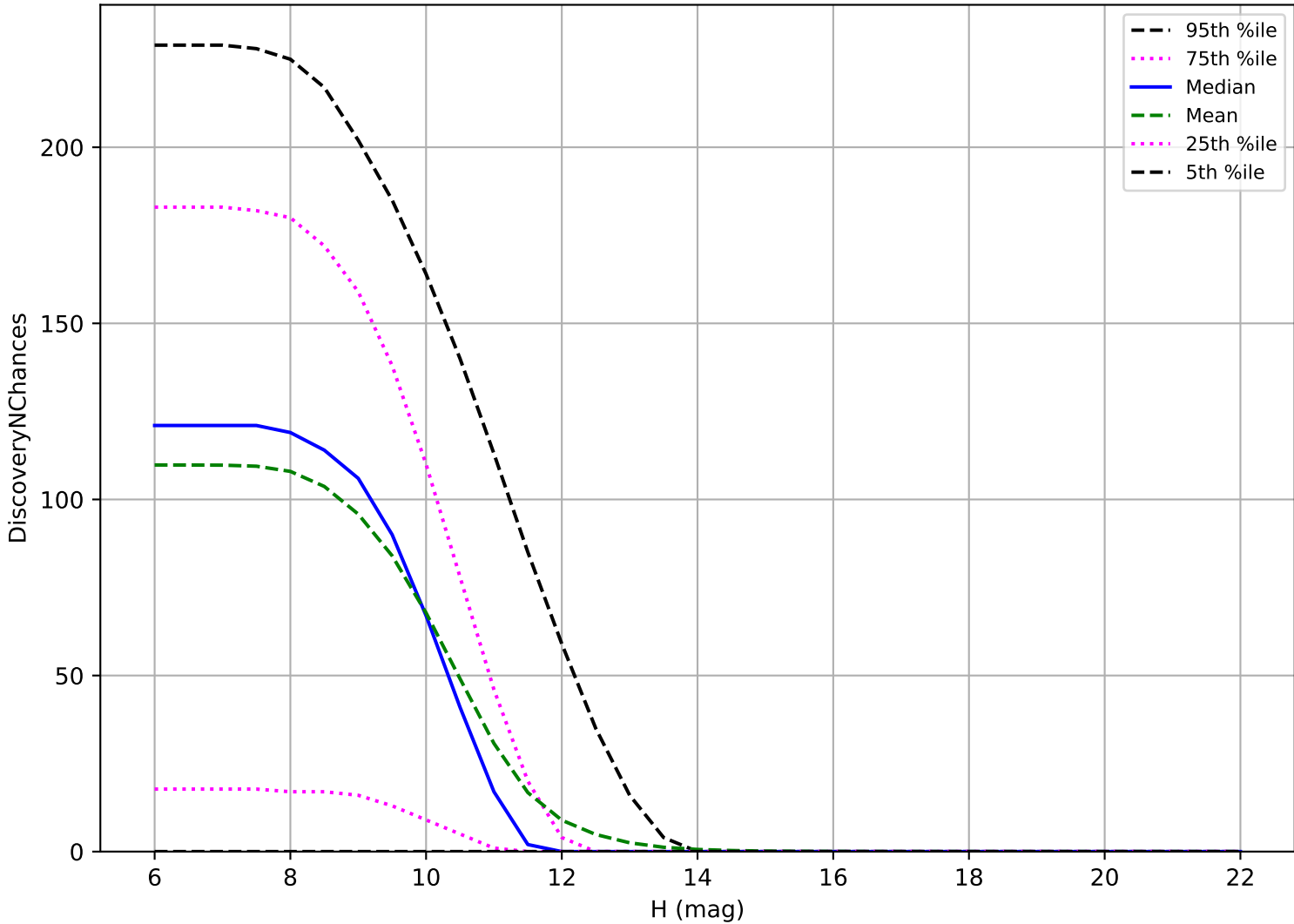
ddf_acor_sf20_lsf30_lsr10_v3.4_10yrs: OCC_r20 3 pairs in 15 nights detection loss
