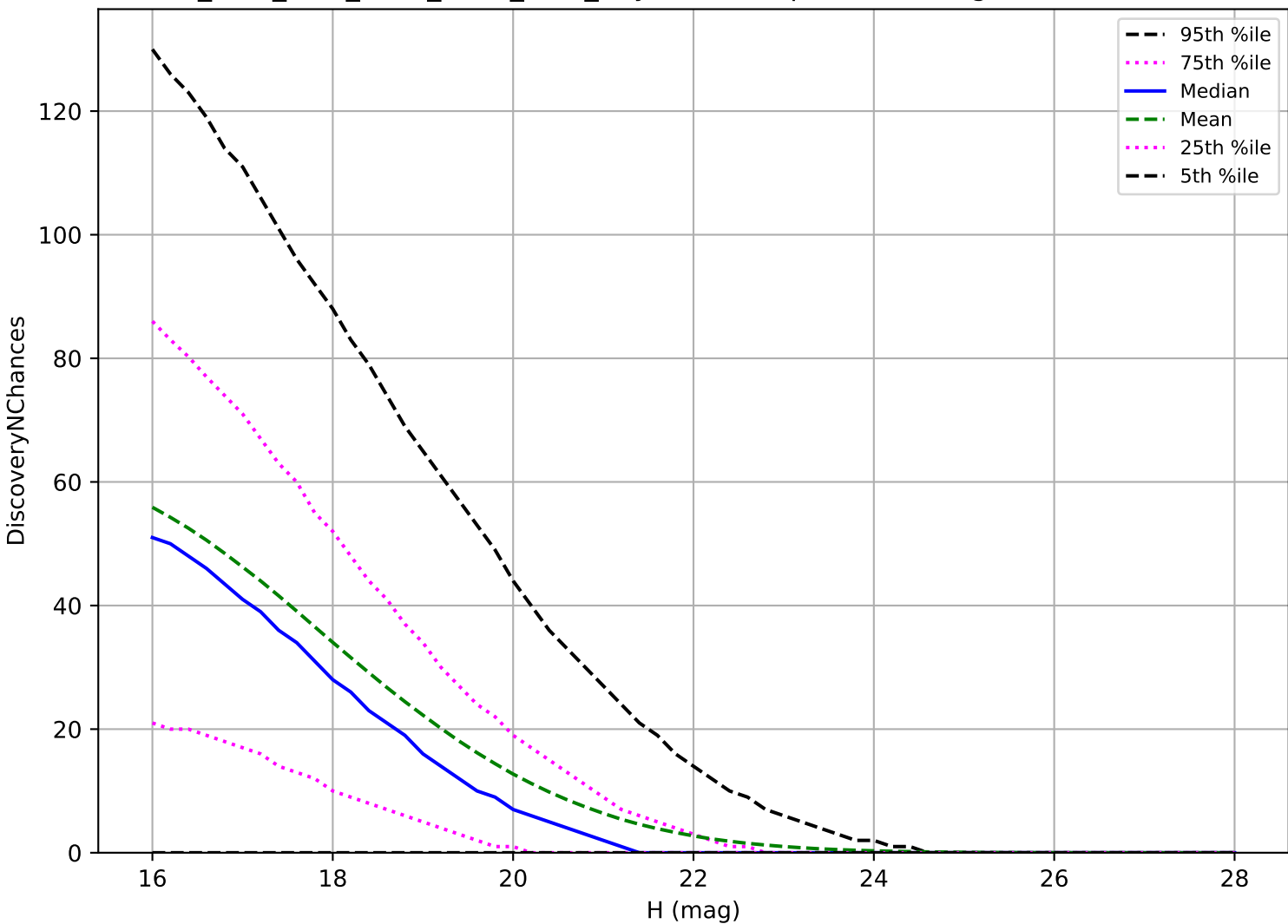
ddf_acor_sf20_lsf30_lsr10_v3.4_10yrs: NEO 3 pairs in 15 nights detection loss
