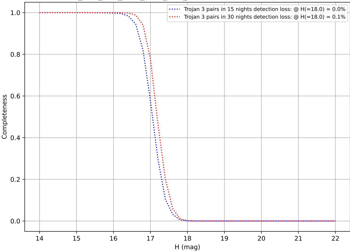
ddf_acor_sf20_lsf30_lsr10_v3.4_10yrs: DifferentialCompleteness
