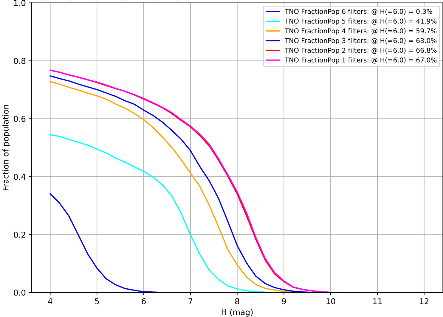
ddf_acor_sf20_lsf30_lsr10_v3.4_10yrs: Fraction of population with colors in X filters TNO
